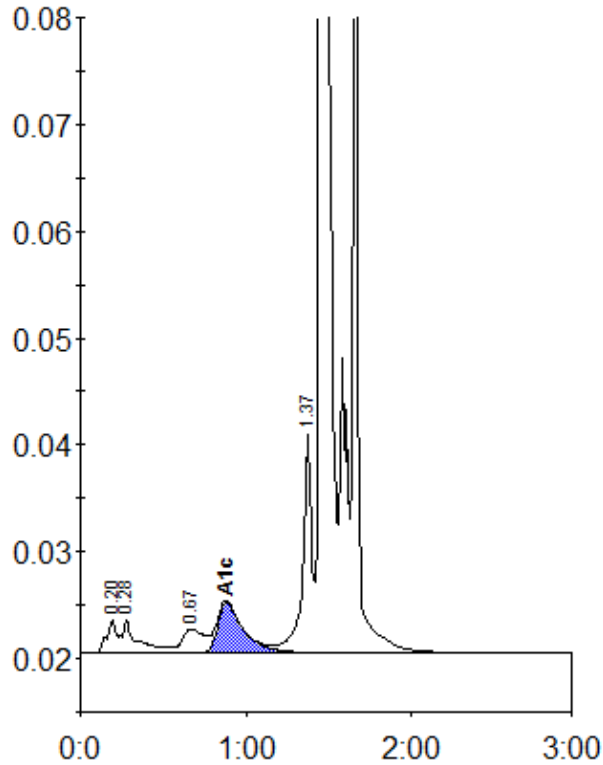
Peak table - ID: 10406970
